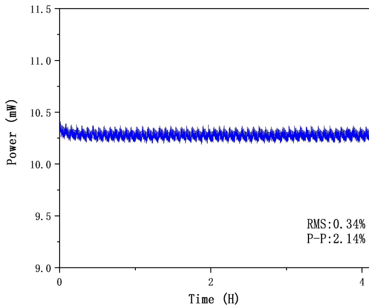
Continuous frequency sweep output power stability
